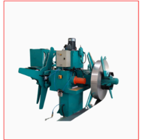
D COILER
