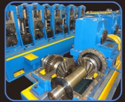
Gear Box
